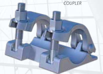
COUPLER
